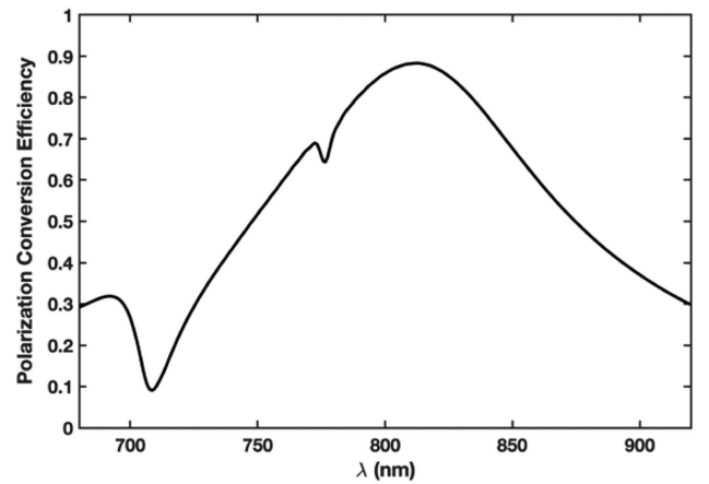
Fig. 5. Numerically simulated polarization conversion efficiency based on the wavelength.
