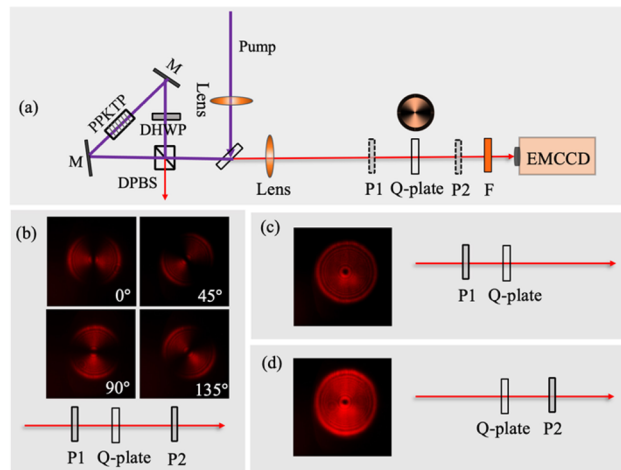
Fig. 1. The directly measured photon distributions in the object arm by an EMCCD. (a) The experimental setup. (b) Photon distribution images with two polarizers, one polarizer placed before the q -plate and the other after the q -plate. The second polarizer P2 is rotated ( 0^\circ , 45^\circ , 90^\circ , 135^\circ ). (c) Photon distribution with only one polarizer, placed before the q -plate. (d) Photon distribution with only one polarizer, placed after the q -plate.
